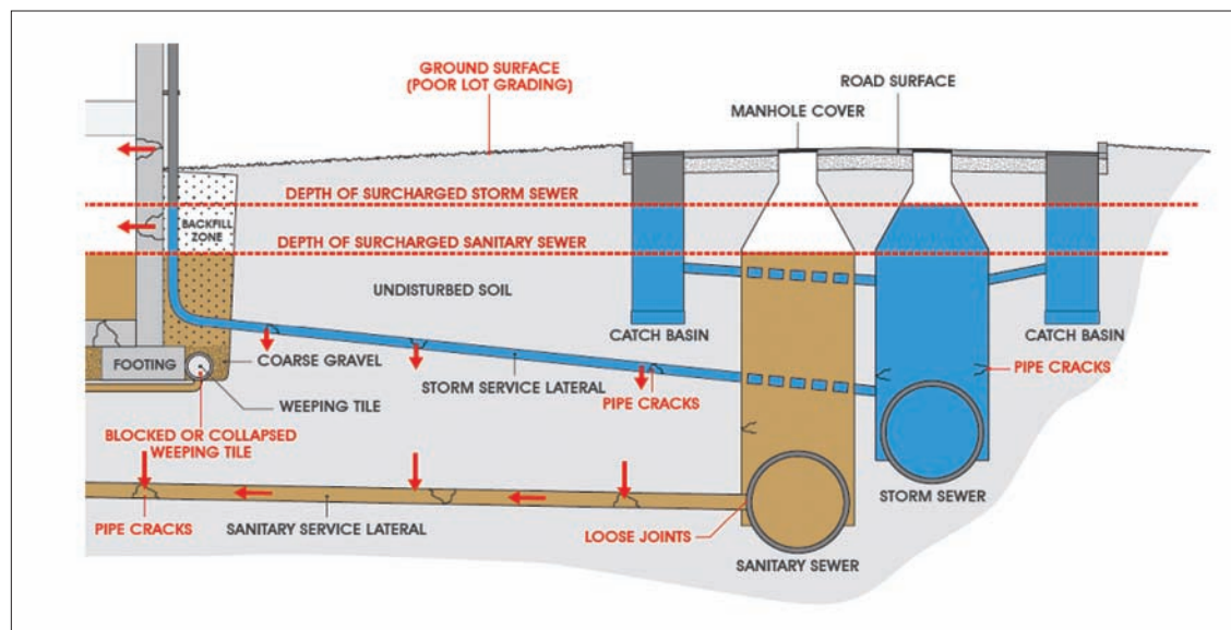
Storm sewer lateral
